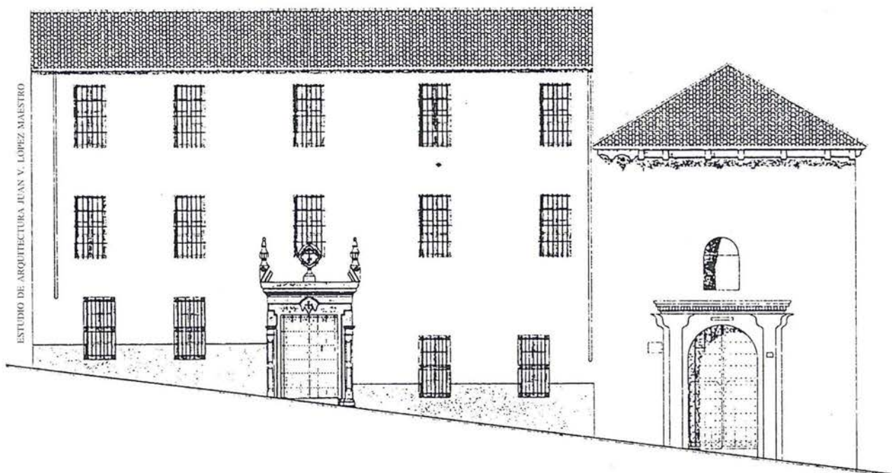
ALZADO PRINCIPAL
